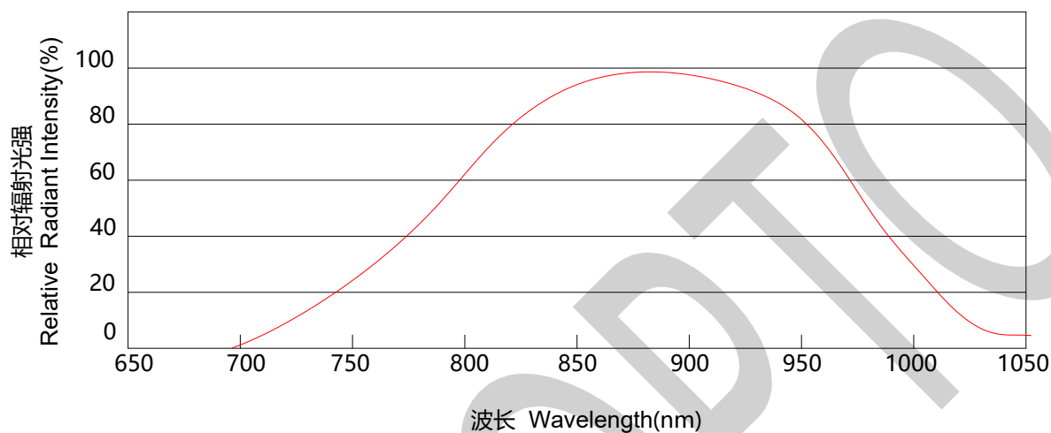
感光特性曲线 Photographic property Curve
